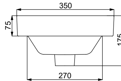
SECTION_VIEW A-A
