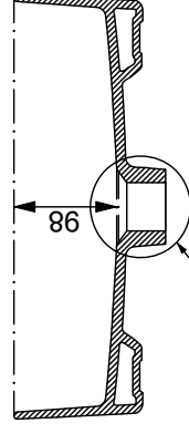
SECTION_VIEW A-A
