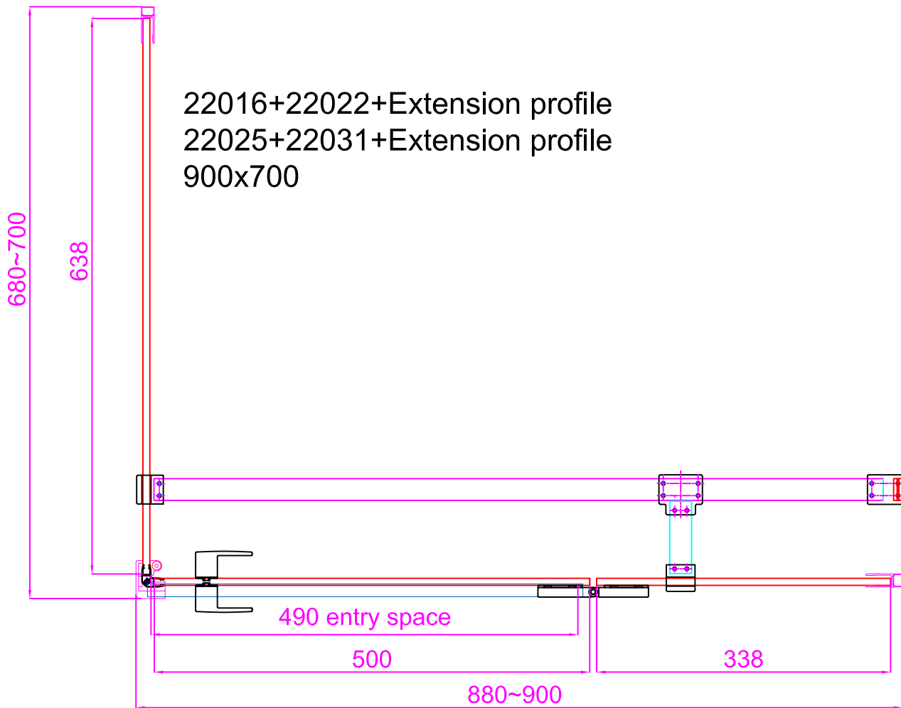
22016/22025 Niche+Extension profile 900
